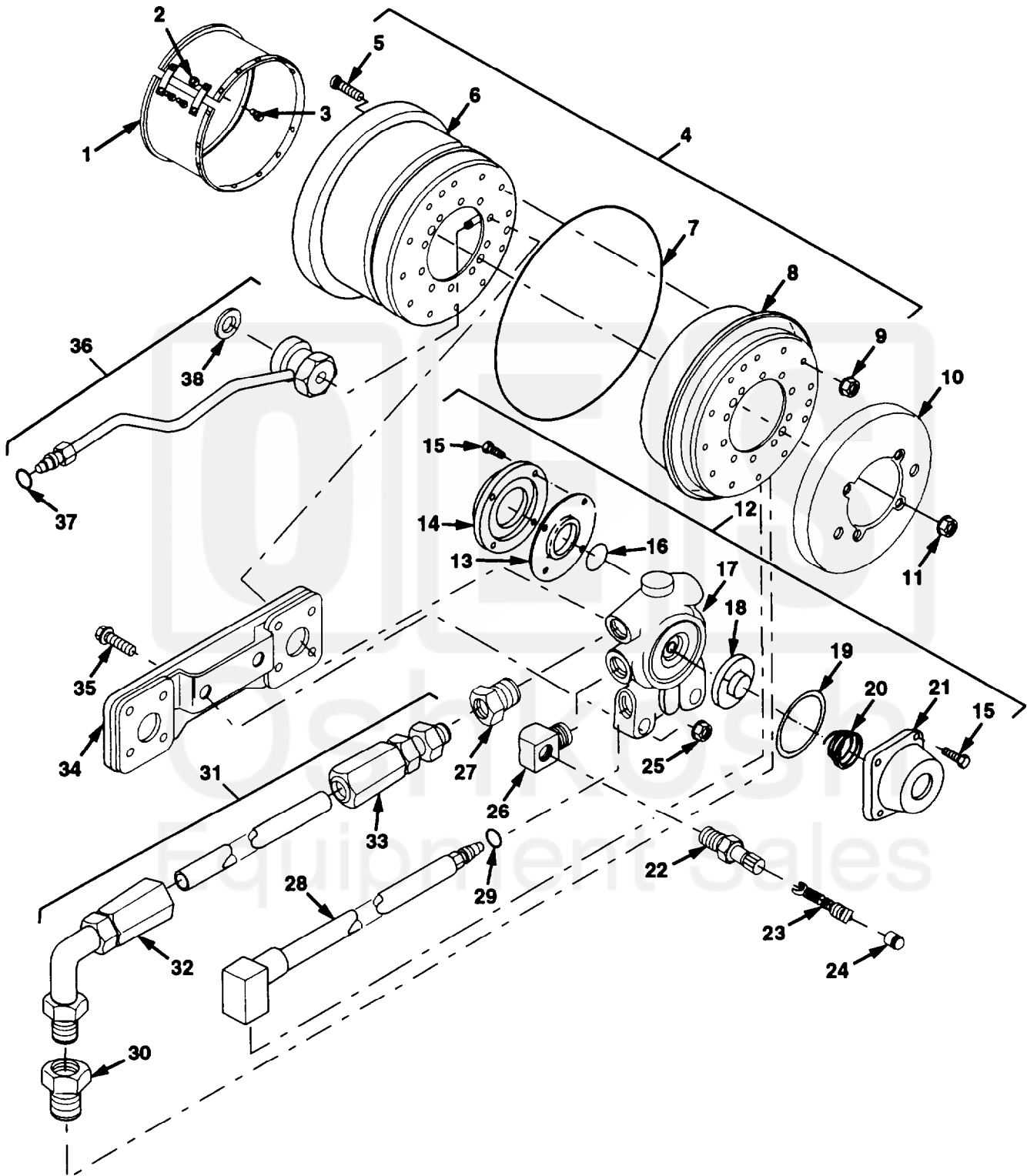
Figure 163. Wheel Assembly
